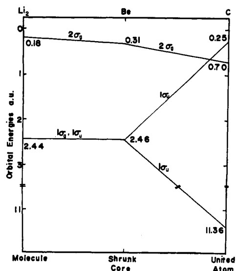
Figure 2a. Orbital energies in united atom, shrunk-core atom † and molecule. Li_2 molecule.
